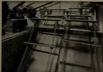
Wood Sliver Conveyers from Grinders in Paper Mill
